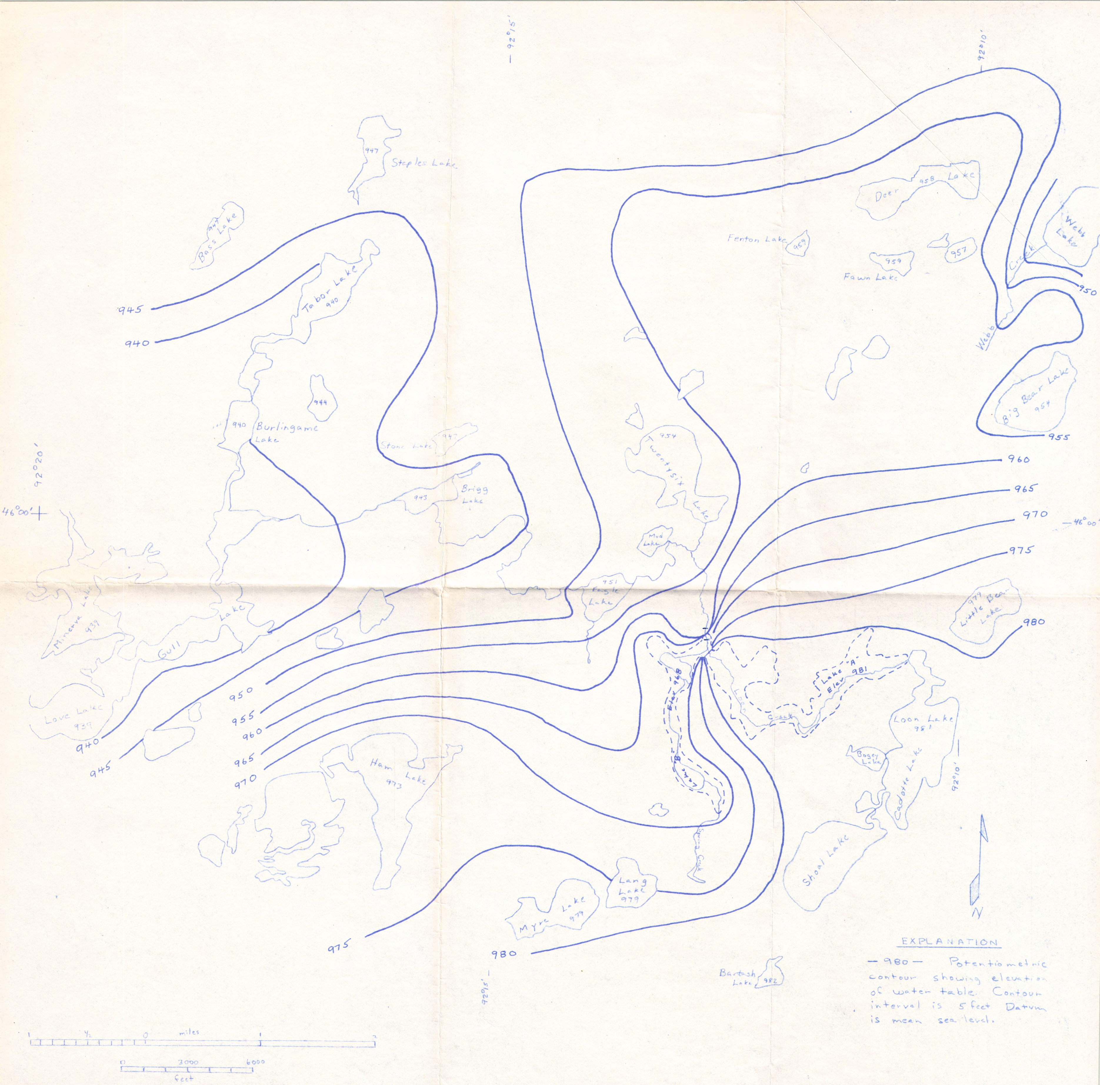
POTENTIOMETRIC MAP OF LOON CREEK AREA SHOWING THE ESTIMATED WATER TABLE WITH PROPOSED RESERVOIRS AT NORMAL OR PLANNED ELEVATIONS
